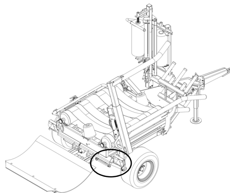
991HS-maskin
